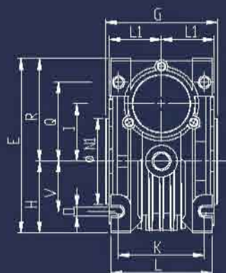
入力軸 INPUT-SHAFT VIEW
