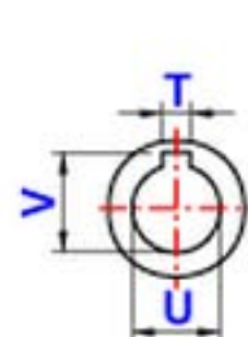
Input-Bore
